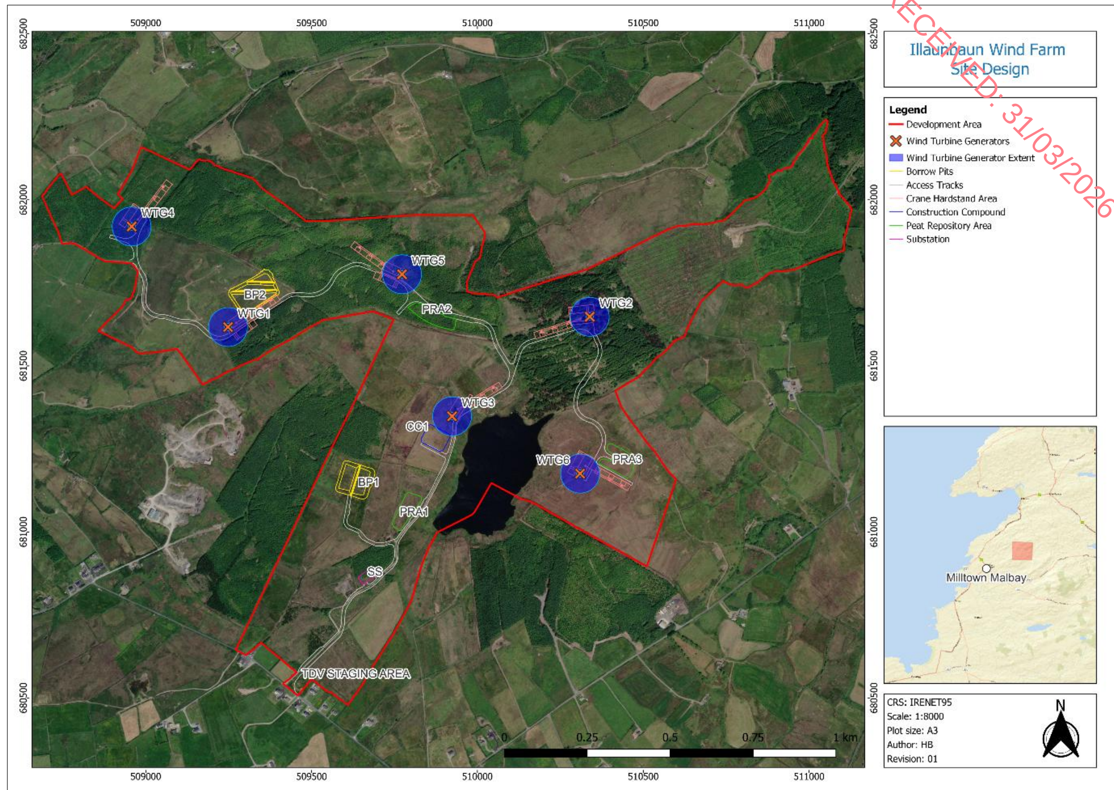
Figure 1-1 Site Layout Plan, with the Slievenalicka Wind Turbine identified as WTG4
